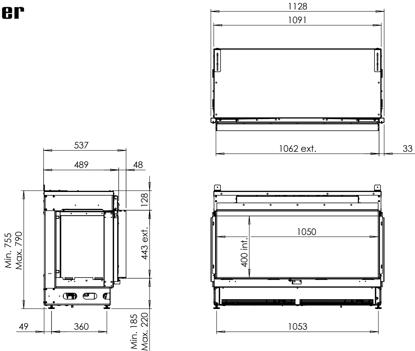
Dimensional Drawing e-Matrix linear 1050/400 I
