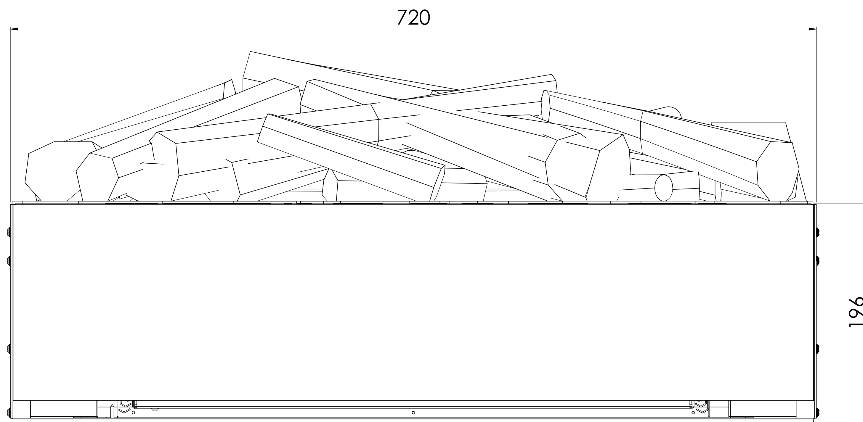
Dimensional Drawing Juneau XL multi
