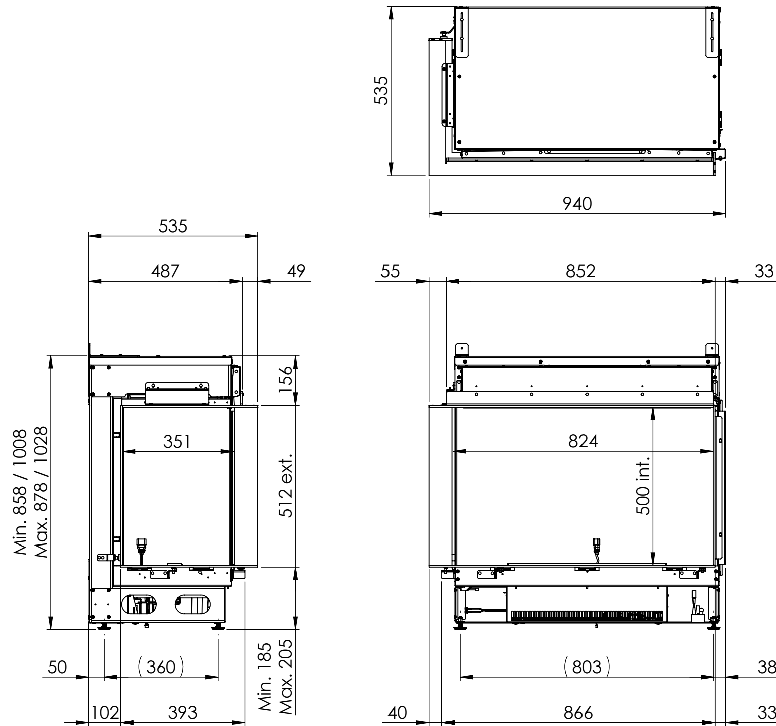
Dimensional drawing e-Matrix 800/500-IIL-RGB
