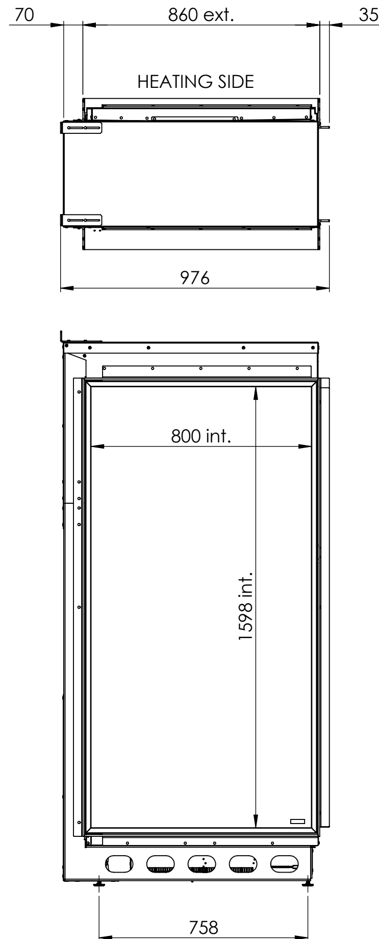
Dimensional drawing e-MatriX 800/1600-ST-RGB
